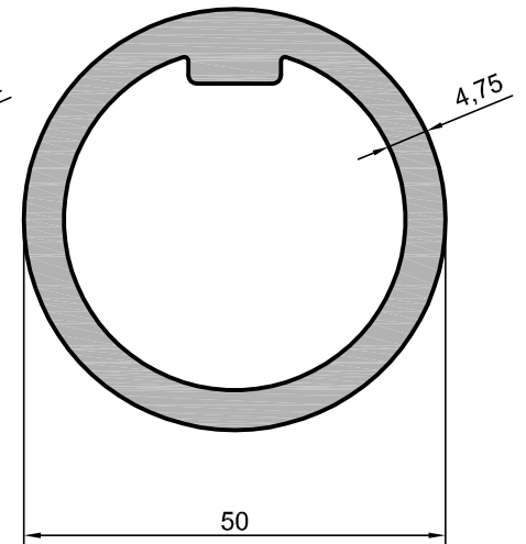
204.31 1,943 kg/m
